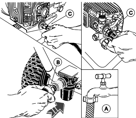
Raccordement hydraulique.
