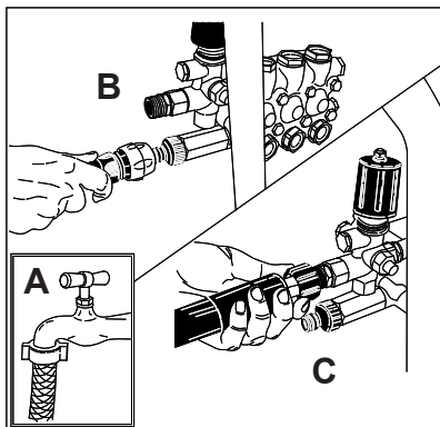
Raccordement hydraulique.
