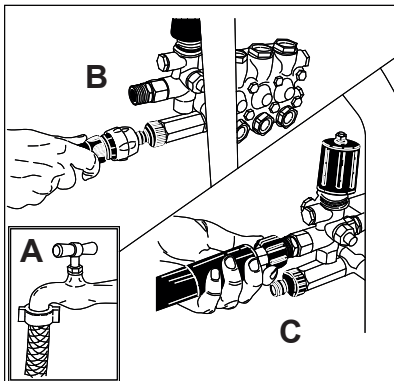
Raccordement hydraulique.
